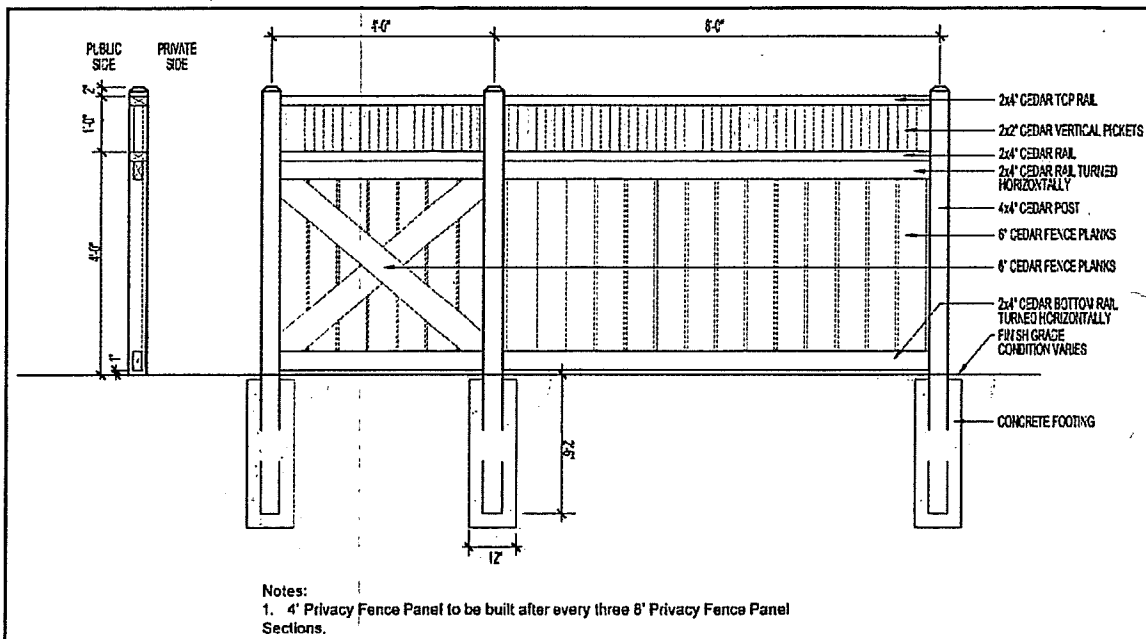
5' PRIVACY FENCE DETAIL
