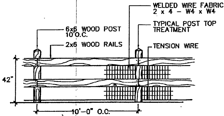
2-RAIL FENCE DETAIL
